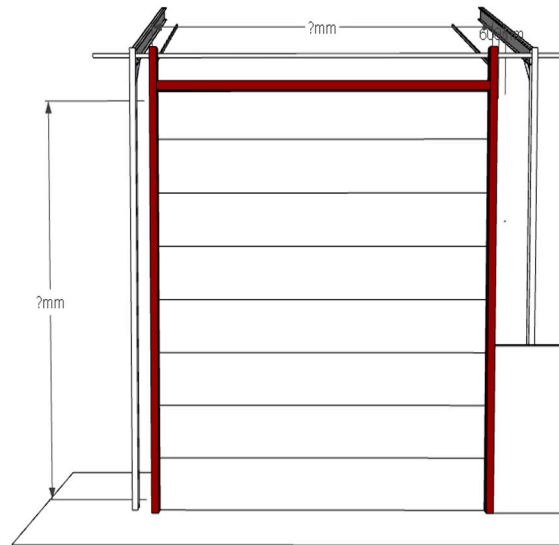
Detail of the face to which we are to fix with information as to what is behind any cladding material because that is what we will fix on to
